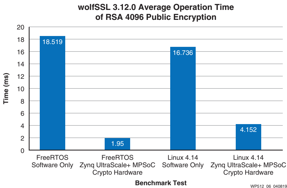
Figure 6: Summary of All RSA-4096 Public Encryption Benchmark Results
