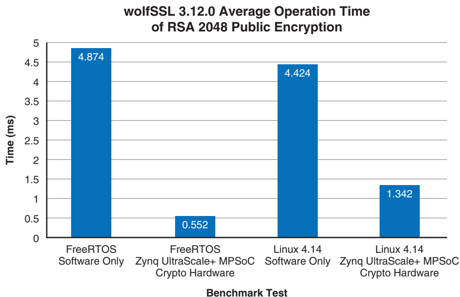
Figure 4: Summary of All RSA-2048 Public Encryption Benchmark Results
