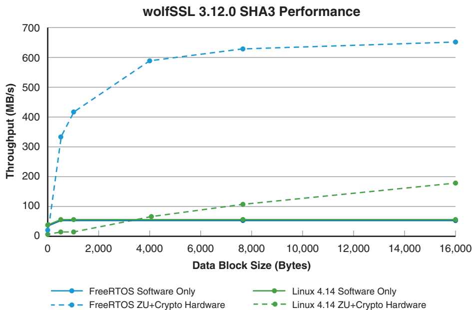
Figure 3: Comparison Summary of All SHA3/384 Results
